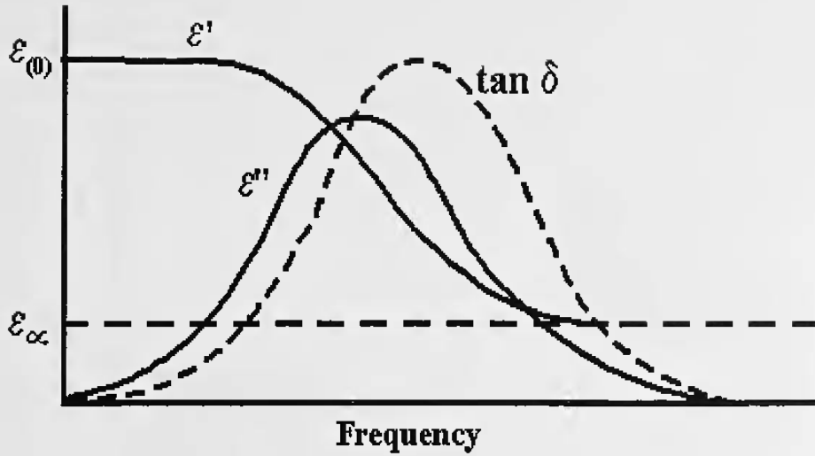
Figure 11. Typical permittivity variation for polar materials.
