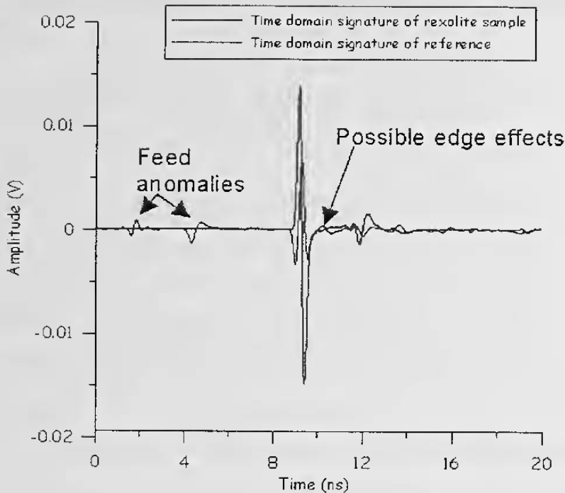
Figure 22. Time-domain data on a Rexolite slab.
